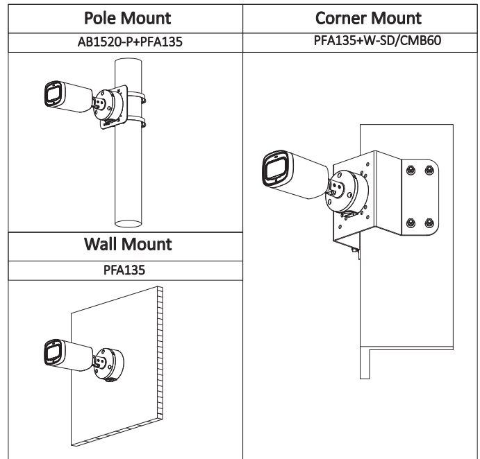
W-SD/CMB60 Corner mount (For use with PFA135 junction box)
